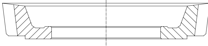
Disc type shaper cutter typical design for cutting external spur gears. The body design may be modified to specific requirements.
