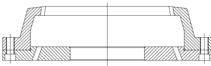
Internal toothed gear shaper cutter for external parts where an interference prevents the use of a conventional disc cutter, and more efficient than a small shank cutter. As with cutters with external teeth these cutters are fully generated to allow resharping throughout the life of the cutter.
