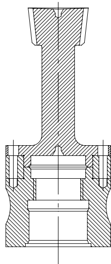
This assembled hub design is produced for small pitch circle diameters cutters where it is not possible to have a hole through the tool, this is necessary to assure the required accuracy.
